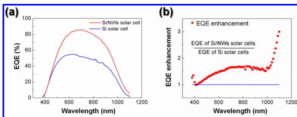
Figure 4. EQE spectra (a) taken from the Si solar cell with \text{In}_x\text{Ga}_{1-x}\text{As} NW array integrated on the back surface, along with the reference Si solar cell; (b) normalized to the reference Si cell.
