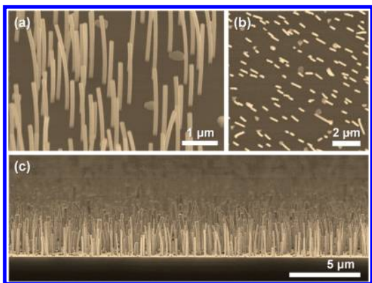
Figure 1. \text{In}_x\text{Ga}_{1-x}\text{As} NW array grown on a Si (111) substrate: (a) 45° tilted SEM image of vertically oriented NWs; (b) top-view SEM image over a 10 \times 10 \text{ }\mu\text{m}^2 area with a number density of \sim 1.4 \times 10^8/\text{cm}^2 ; and (c) panoramic view of a cross-section SEM image of the NWs with a height of ca. 2–3 \mu\text{m} .
