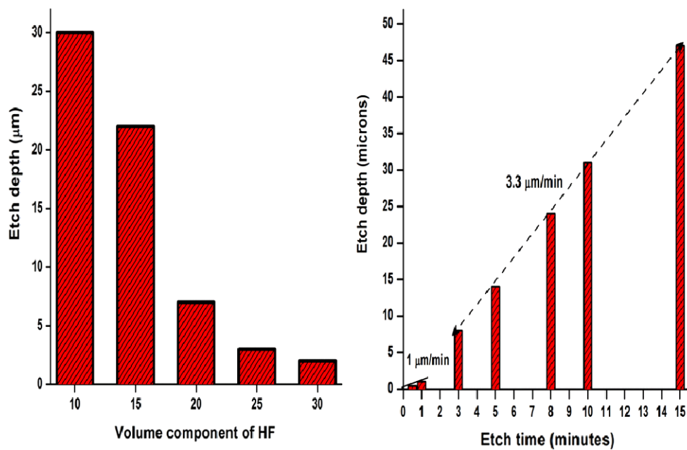
Figure 5. Variation of etch rate with chemical composition and etch time. (Left) Etch depth as a function of volume component ( x ) of HF for p^+ (resistivity = 0.001–0.005 \Omega cm and diameter \sim 60–80 nm) nanowires etched for 10 min in x :1:3 ([HF]/[H 2 O 2 ]/[ethanol]) recipes. The etch depth decreases with higher volume components of HF. (Right) Etch depth as a function of etch time for 60–80 nm p^+ nanowires produced using the 10:1:3 ([HF]/[H 2 O 2 ]/[ethanol]) recipe. The variation of etch depth follows a linear trend (as shown by the dashed line with arrows) after the first few minutes.
