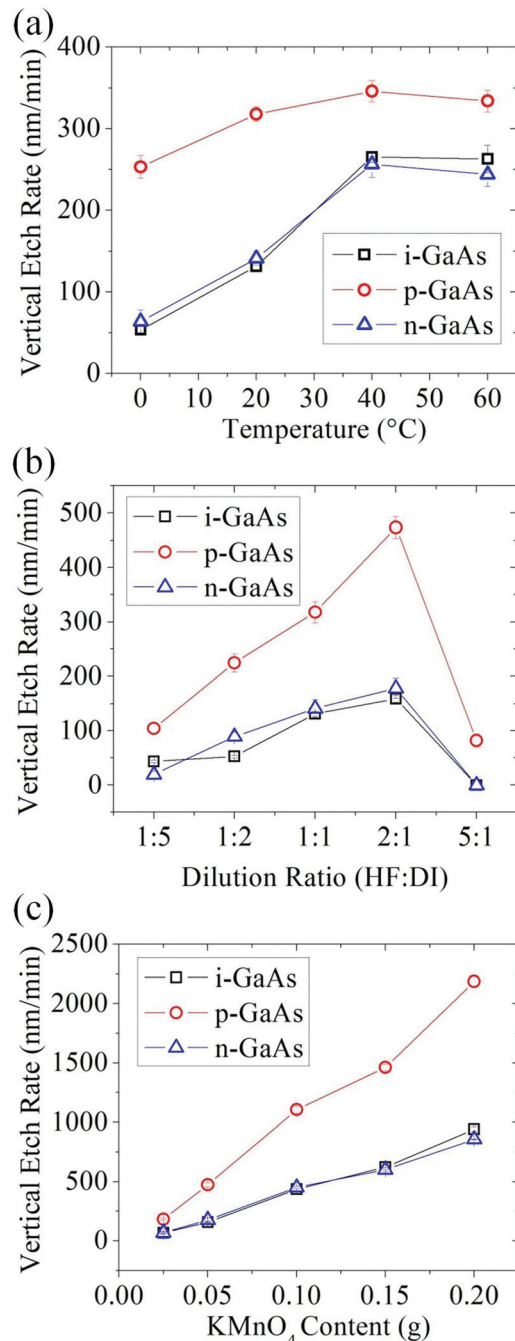
FIG. 2. Quantification of VER as a function of (a) solution temperature, (b) acid dilution ratio, and (c) oxidant concentration. Etch rates for p-, i-, and n-GaAs samples are represented by red circles, black squares, and blue triangles, respectively. Each data point represents mean VER values obtained from sample sets of 25 nanopillars (with vertical sidewall structures), while error bars represent \pm one standard deviation from the mean.
